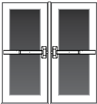
Two rim devices with mullion — same direction
